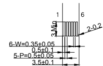
△ Detail " B " Scale 5:1
